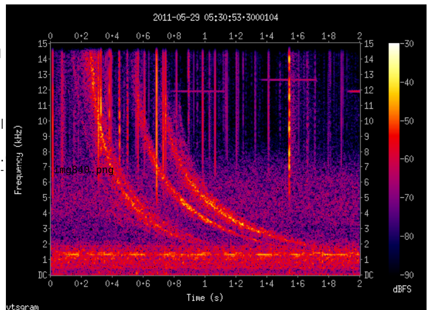
A strong whistler set against a background of natural VLF hiss.
