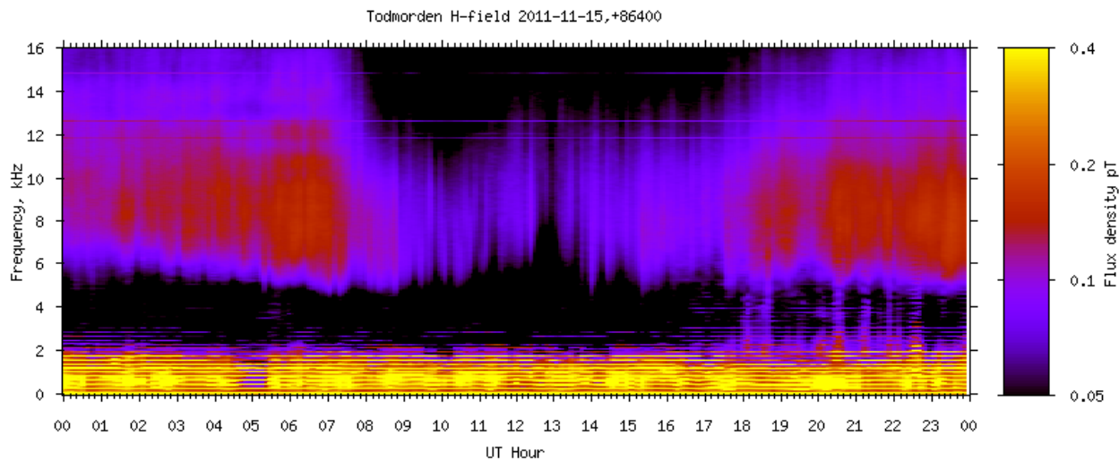
A 24 hour spectrogram, produced by vtindex into gnuplot pm3d , shows a typical diurnal variation of sferic activity.
