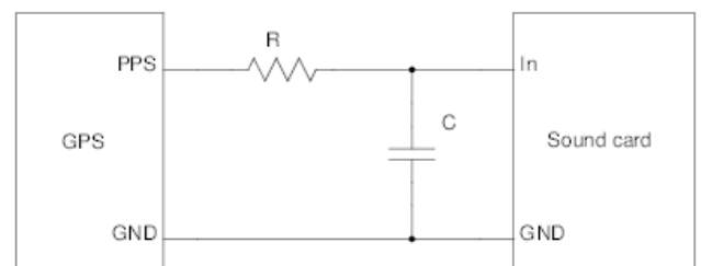
A simple RC low pass filter to shape the PPS.
