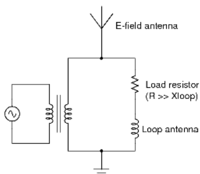
General scheme for a calibrator to align E-field and H-field phase response. The AC source is stepped up to a high voltage via the transformer, which produces an electric field. Current through the load resistor produces a magnetic field in the loop which is almost in phase with the electric field.
