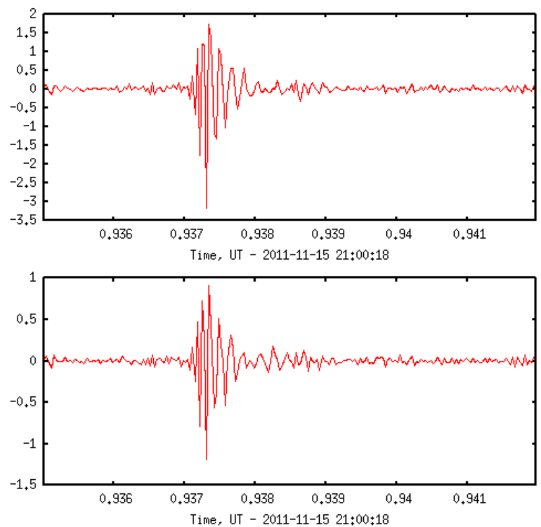
A sferic received by a pair of loop antennas, rendered by vtplot.
